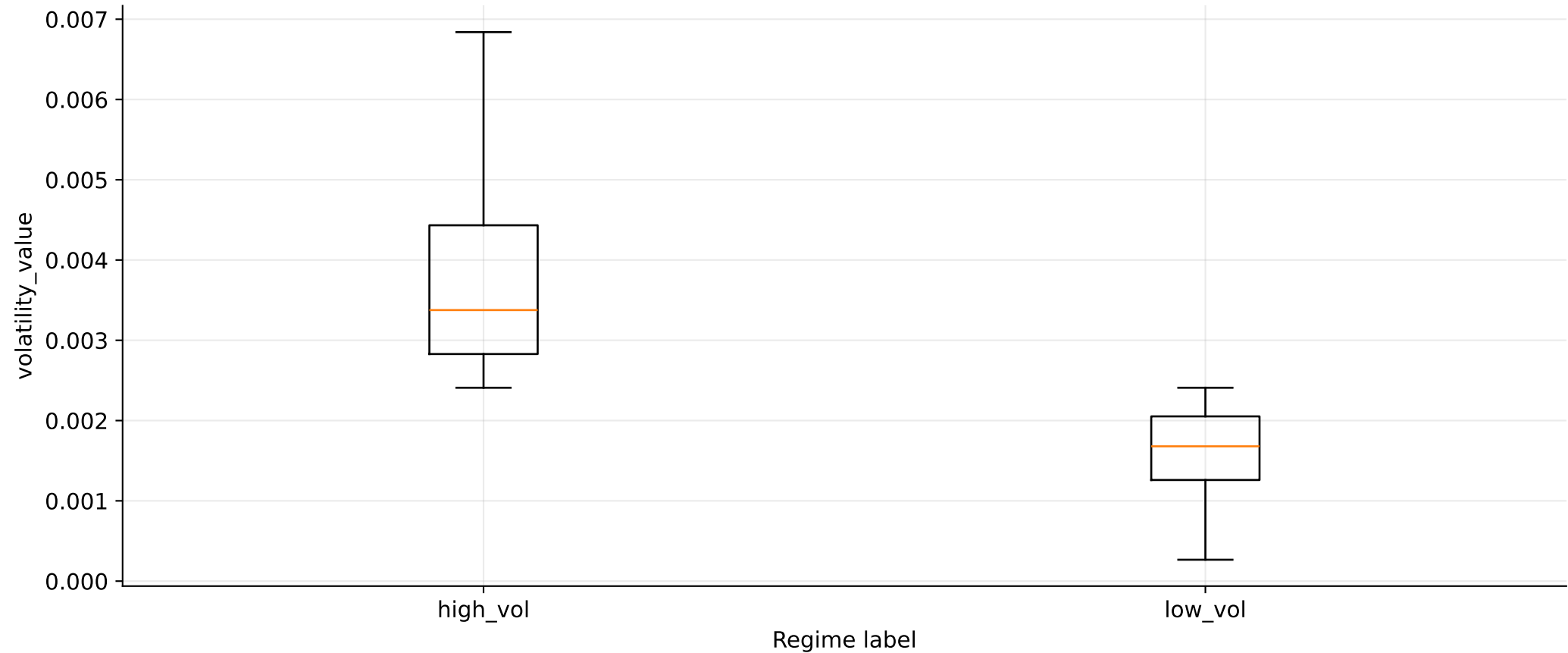
Volatility distribution by regime - BTCUSDT 15m quantile
